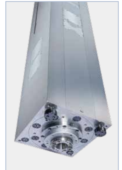
Available to equip with a highly rigid square ram type spindle head on Z-axis (optional).
