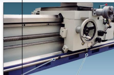
▶ 第三支撐面，增強大工件 切削強度 The 3rd rail enhance the cutting force. ▶ 自動定寸切削裝置 Longitudinal Stop Device.
