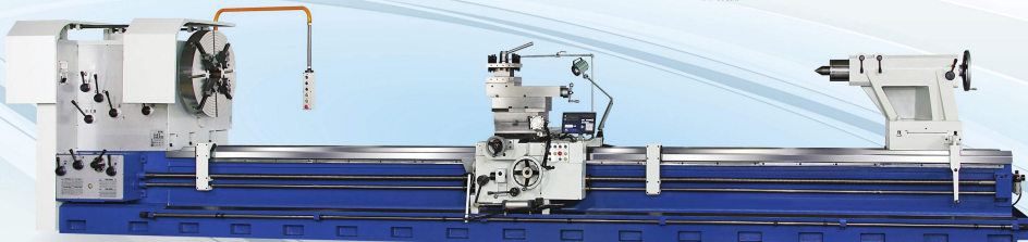
◆ Pin-locking type 4-way tool post ensures safety in cutting and is easy to swivel forward and reversely. 插銷式四方刀架，可確保四方刀架反 向切向時滑動以確保安全，且方便正 反向轉動。
